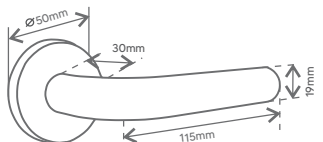
Marine Color 01 - Redonda Grande
