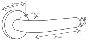
Marine 01 - Redonda Grande
